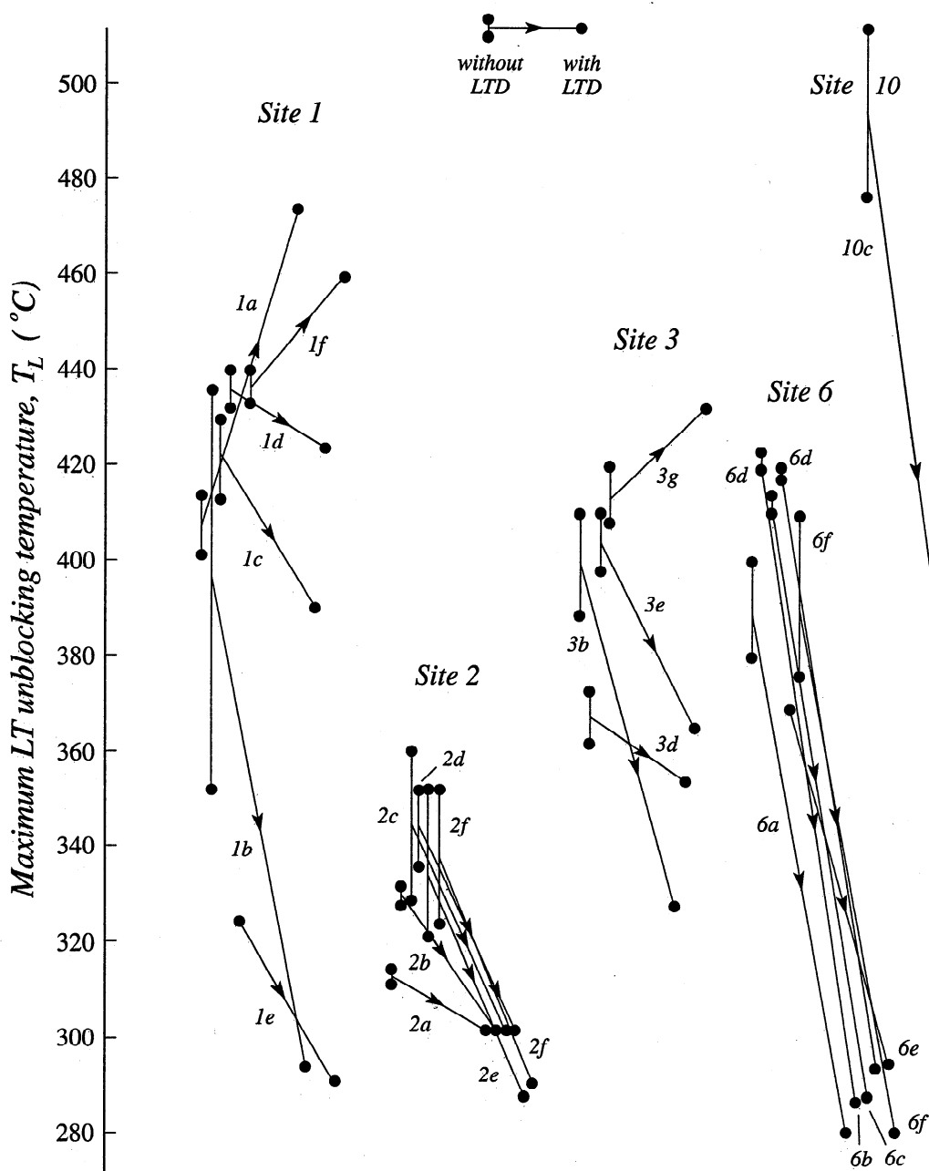
Figure 8. A sample-by-sample comparison of T_L values without LTD (left-hand points in each pair, usually two specimens) and with LTD (right-hand point, one specimen), as indicated by the model at top. In all but three instances, T_L decreases as a result of LTD, and in many cases (every sample for sites 2 and 6), the T_L value following LTD is in the range expected for single-domain grains ( \sim 300^\circ\text{C} ).
