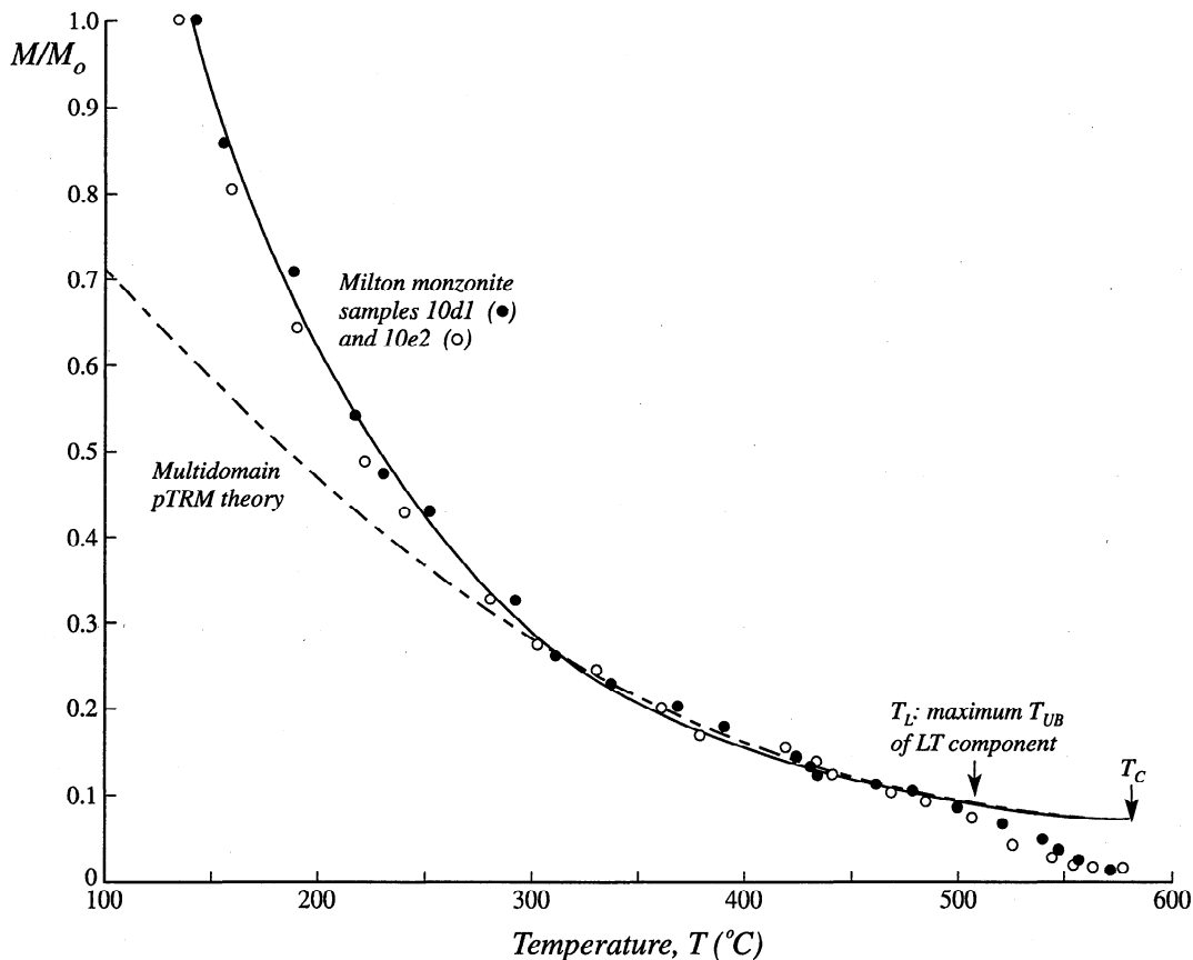
Figure 3. Thermal demagnetization of two samples from site 10, where LT is carried by truly multidomain grains and HT is very small compared to LT. The demagnetization tails off exponentially and agrees with predictions of multidomain partial TRM theory [Dunlop and Xu, 1994]. The final decrease in magnetization just below T_C is due to demagnetization of the small HT vector.
