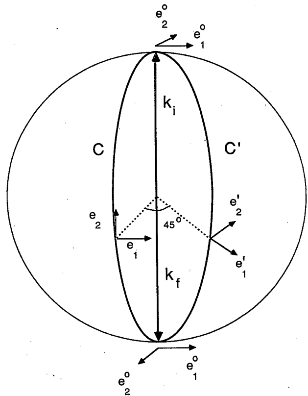
FIG. 5. When the individual scattering angles are small, the wave vectors \mathbf{k}_j define a nearly continuous curve on the sphere of radius k_0 . The polarization vector of the wave is parallel transported along this curve. For example, curve C corresponds to a scattering path for light with incident wave vector \mathbf{k}_i and final wave vector \mathbf{k}_f = -\mathbf{k}_i . Parallel transport of the unit vectors \hat{\mathbf{e}}_1 and \hat{\mathbf{e}}_2 along path C leads to inversion of \hat{\mathbf{e}}_2 , while \hat{\mathbf{e}}_1 is preserved. Thus, if the polarization of the incident light is directed along either \hat{\mathbf{e}}_1 or \hat{\mathbf{e}}_2 , then path C would lead to observed light polarized along the same direction. Parallel transport along the path C' , obtained from C by rotation through 45^\circ about the incident wave vector, would lead to transposition of \hat{\mathbf{e}}_1 and \hat{\mathbf{e}}_2 . This path would contribute to the perpendicular polarization channel, if the incident light is directed along \hat{\mathbf{e}}_1 or \hat{\mathbf{e}}_2 . In general, for any path C contributing to the parallel polarization channel, there is a path C' obtained as above, which contributes to the opposite polarization channel.
