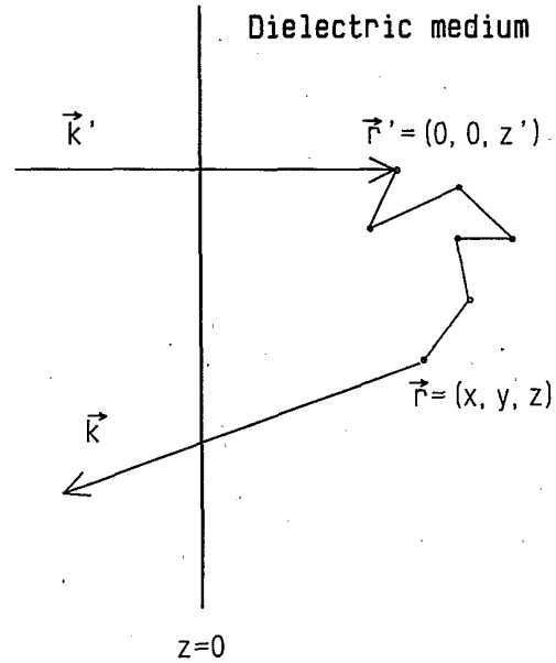
FIG. 1. A typical multiple-scattering path. The incident wave with wave vector \mathbf{k}' begins to scatter at \mathbf{r}' = (0, 0, z') . The kernel L(\mathbf{r}, \mathbf{r}'; \mathbf{k}, \mathbf{k}'; t) describes the transport of the field from \mathbf{r}' to \mathbf{r} within the medium. The coherent field from \mathbf{r} = (x, y, z) is then observed as the reflected light.
