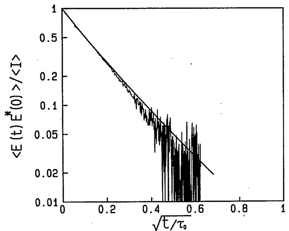
FIG. 4. In the crossed linear polarization channel, the elimination of short scattering paths leads to much better agreement with the observed autocorrelation function. The increased slope in both the observed and calculated correlation functions is due to the fact that short paths, which tend not to flip the polarization, do not contribute in this channel.
