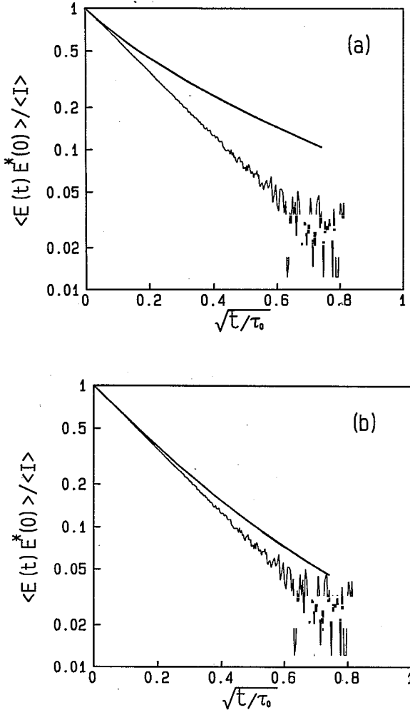
FIG. 2. (a) The autocorrelation function in the scalar white-noise model for isotropic scattering deviates dramatically from the observed nearly straight-line exponential behavior. At long times t \sim \tau_0 , the overestimate of short paths leads to a much slower decay than is observed. (b) The simple correction derived in Sec. V improves the agreement with the observed exponential behavior. Physically, this is due to a more realistic treatment of short paths.
