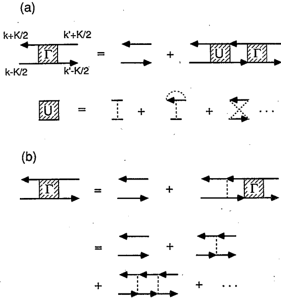
FIG. 3. (a) The Bethe-Salpeter equation is an integral equation relating the transport kernel \Gamma to the irreducible vertex function U . The irreducible vertex is defined as the sum of all diagrams which do not fall into two distinct parts when a single pair of retarded and advanced propagators (solid lines) are cut. The first few terms in U have been shown. The last of these is one of the "maximally crossed" diagrams. (b) In the weak scattering approximation, only the first term in the expansion of U is included. The Bethe-Salpeter equation then reduces to the sum of ladder diagrams.
