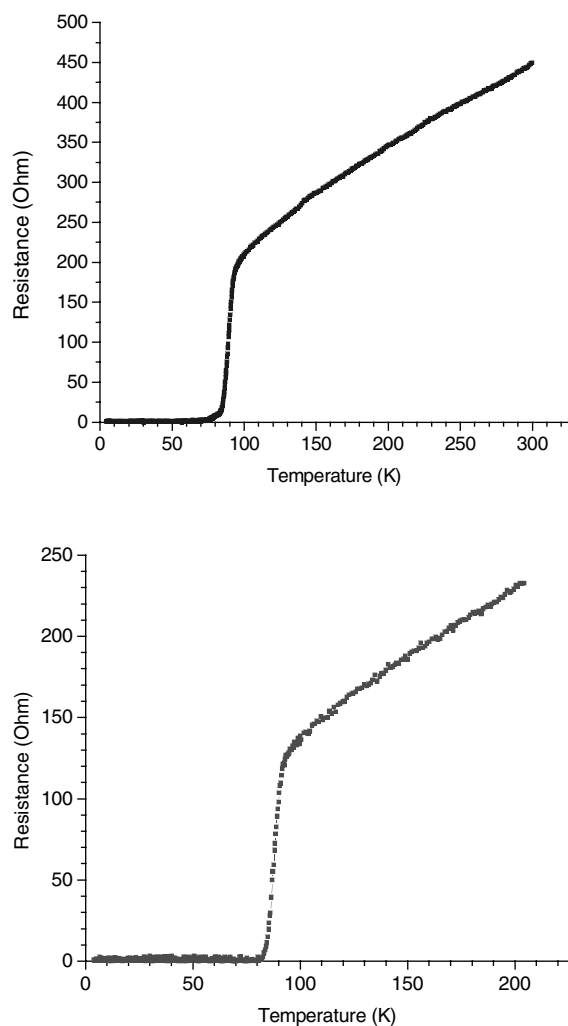
Fig. 3. Electrical characterization of two (optimally-doped \text{YBa}_2\text{Cu}_3\text{O}_7 ) nanowires shows high-temperature superconductivity at critical temperatures of 89 and 87 K, both with sharp ( \sim 3 K) transitions. This authenticates the cleanliness of our nanofabrication process.
