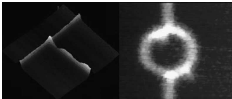
Fig. 2. (Left) An AFM picture of a Y-junction of optimally-doped YBCO (width: 60 nm, thickness: 20 nm). (Right) An Aharonov–Bohm ring of underdoped cuprate by the novel fabrication technique of nanomachining. The diameter of the ring (1.6 \mu\text{m} ) corresponds to a flux periodicity ( h/e ) of roughly 20 Gauss. Because of its size, the structure is capable of sensitive detection of single vortex-like (vison) motion. In a similar structure grown below the underdoped regime, the charge of the carriers can be accurately determined by interference measurement as e , 2e or any fraction thereof.
