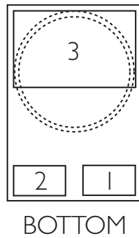
Figure 9a. LUXEON Rebel Color Line pad configuration.
