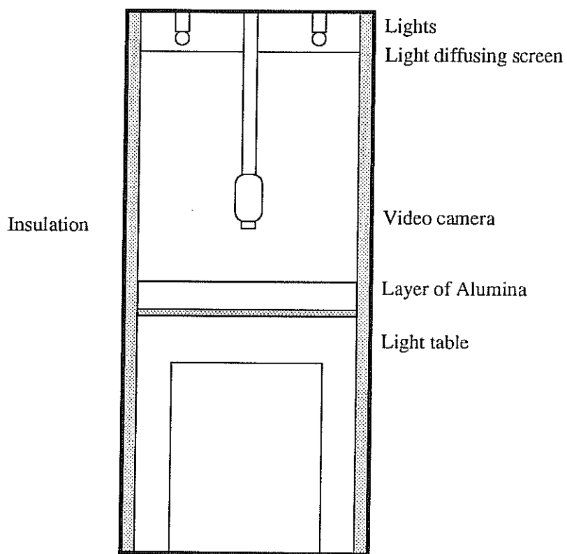
Figure 2.1: The experimental apparatus.
