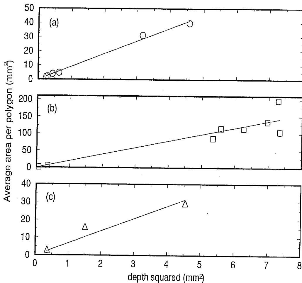
Figure 3.13: A_p as a function of d^2 with linear fits forced through the origin. The error bars are the same size as the symbols. (a) Type A experiments; A_p = (9.02 \pm 0.26)d^2 , (b) Type B experiments; A_p = (19.5 \pm 1.7)d^2 , (c) Type C experiments; A_p = (6.89 \pm 0.88)d^2 .
