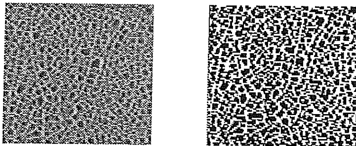
Figure 3.3: Greyscale and black and white images of an 8 cm \times 8 cm region of the crack pattern for a Type A experiment with d = 0.54 \pm 0.02 mm.
