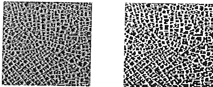
Figure 3.4: Greyscale and black and white images of an 8 cm \times 8 cm region of the crack pattern for a Type A experiment with d = 0.66 \pm 0.02 mm.
