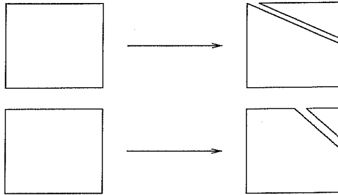
Figure 3.34: Illustration of how polygons split
