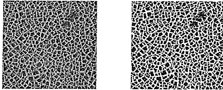
Figure 3.9: Greyscale and black and white images of an 8\text{ cm} \times 8\text{ cm} region of the crack pattern for a Type C experiment with d = 0.60 \pm 0.02\text{ mm} .
