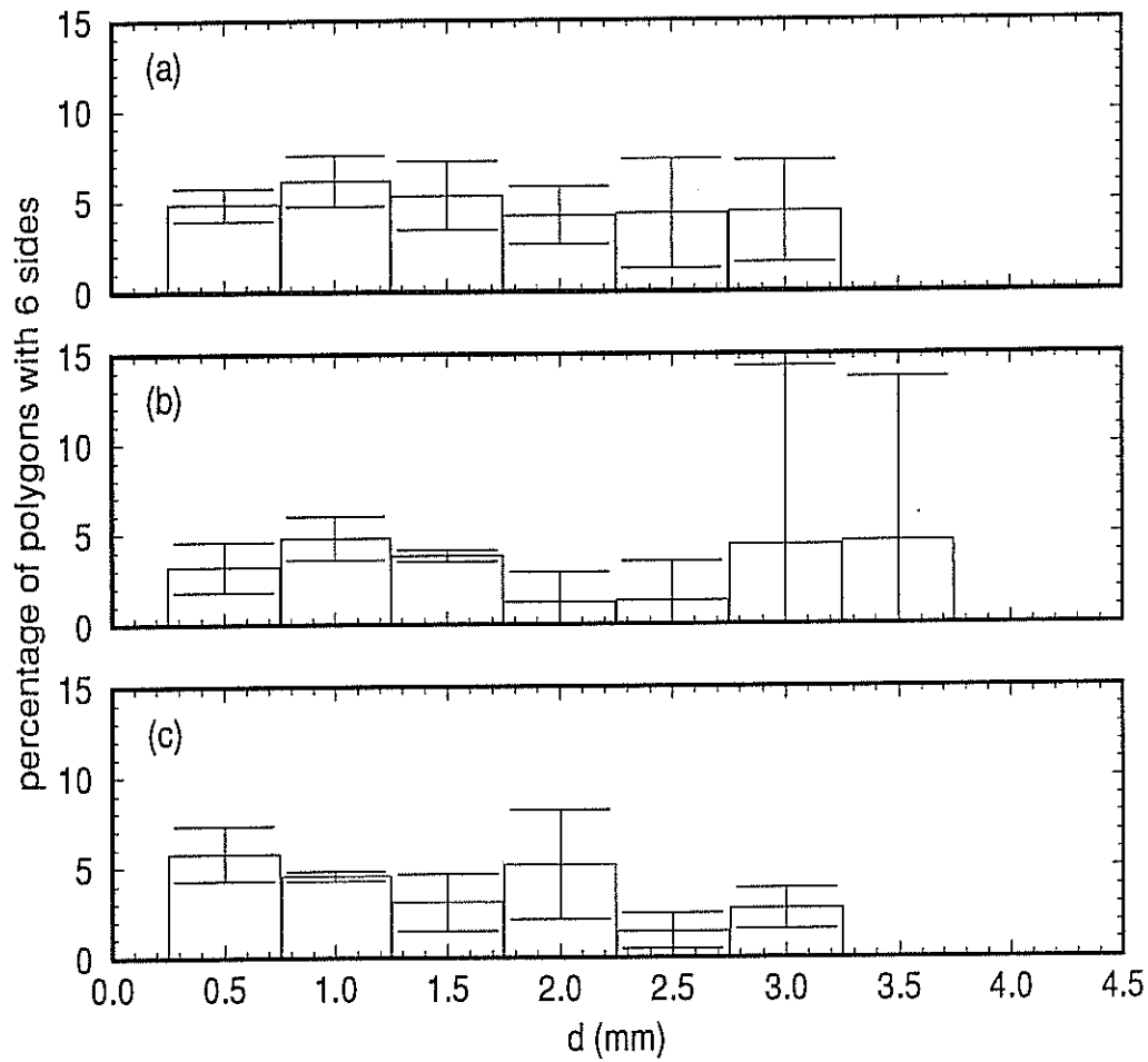
Figure 3.33: Percentage of six sided polygons as a function of d . (a) Type A experiments, (b) Type B experiments, (c) Type C experiments.
