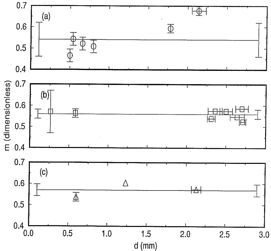
Figure 3.12: The fraction of area which is solid, m as a function of d . The straight line is the mean of the data and the error bars on the lines are the standard deviation of that mean. (a) Type A experiments; \bar{m}_A = 0.541 \pm 0.080 , (b) Type B experiments; \bar{m}_B = 0.560 \pm 0.021 , (c) Type C experiments; \bar{m}_C = 0.570 \pm 0.028 .
