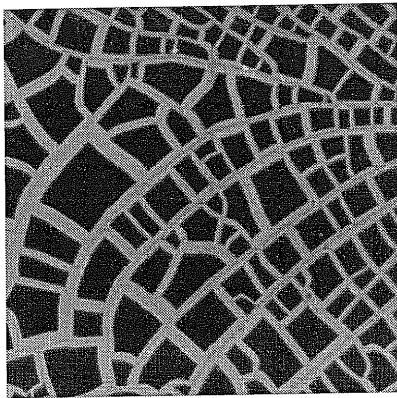
Figure 3.37: Pattern formed in a Type B experiment. d = 2.51 \pm 0.17 mm
