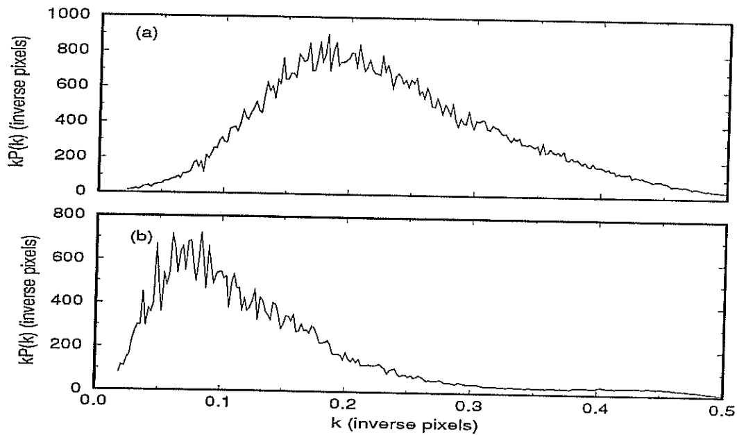
Figure 3.17: Azimuthally averaged power spectra of Type A experiments, (a) d = 0.49 \pm 0.07 mm, (b) = 1.93 \pm 0.21 mm.
