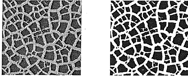
Figure 3.11: Greyscale and black and white images of an 8 cm \times 8 cm region of the crack pattern for a Type C experiment with d = 2.13 \pm 0.06 mm.
