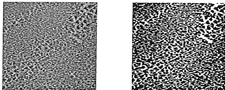
Figure 3.6: Greyscale and black and white images of an 8 cm \times 8 cm region of the crack pattern for a Type B experiment with d = 0.26 \pm 0.02 mm.
