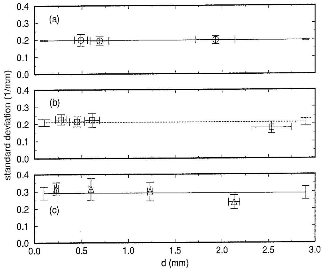
Figure 3.23: The standard deviation \sigma as a function of d . The lines are the mean value, \bar{\sigma} and the error bars on the lines are the standard deviation. (a) Type A experiments; \bar{\sigma} = 0.197 \pm 0.003 \text{ mm}^{-1} , (b) Type B experiments; \bar{\sigma} = 0.210 \pm 0.022 \text{ mm}^{-1} , (c) Type C experiments; \bar{\sigma} = 0.292 \pm 0.037 \text{ mm}^{-1} .
