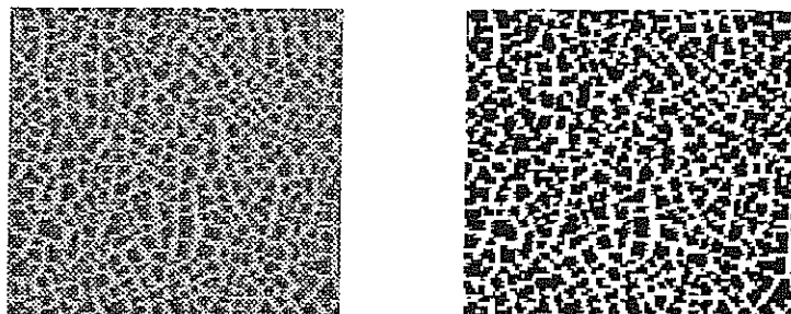
Figure 3.7: Greyscale and black and white images of an 8 cm \times 8 cm region of the crack pattern for a Type B experiment with d = 0.58 \pm 0.02 mm.
