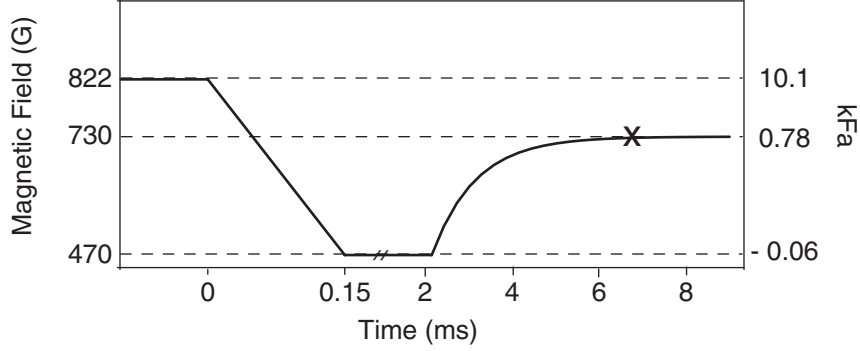
Figure 6-4: Experimental sequence of the magnetic field ramp. Ramp down speed is limited by the clamp voltage of the varistor used and ramp up speed is limited by the maximum voltage of our power supplies. Also shown is the inverse interaction parameter k_{Fa} corresponding to each magnetic field for the Kapitza-Dirac experiment.
