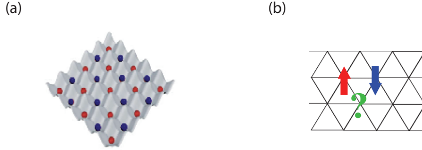
Figure 7-3: Visualizations of (a) antiferromagnetic ordering in a square lattice and (b) spin frustration in a triangular lattice.
