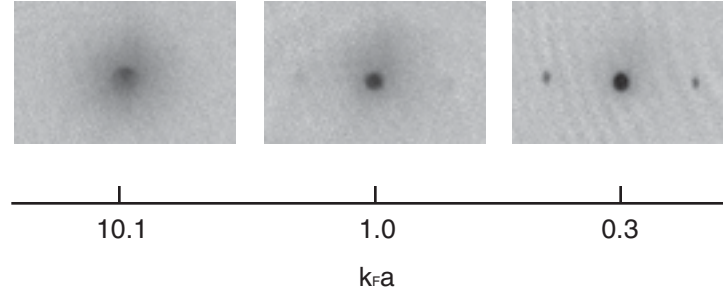
Figure 6-5: Visibility of distinct momentum peaks for different k_F a . Within the strongly interacting regime ( k_F a large), the different momentum peaks are smeared out.
