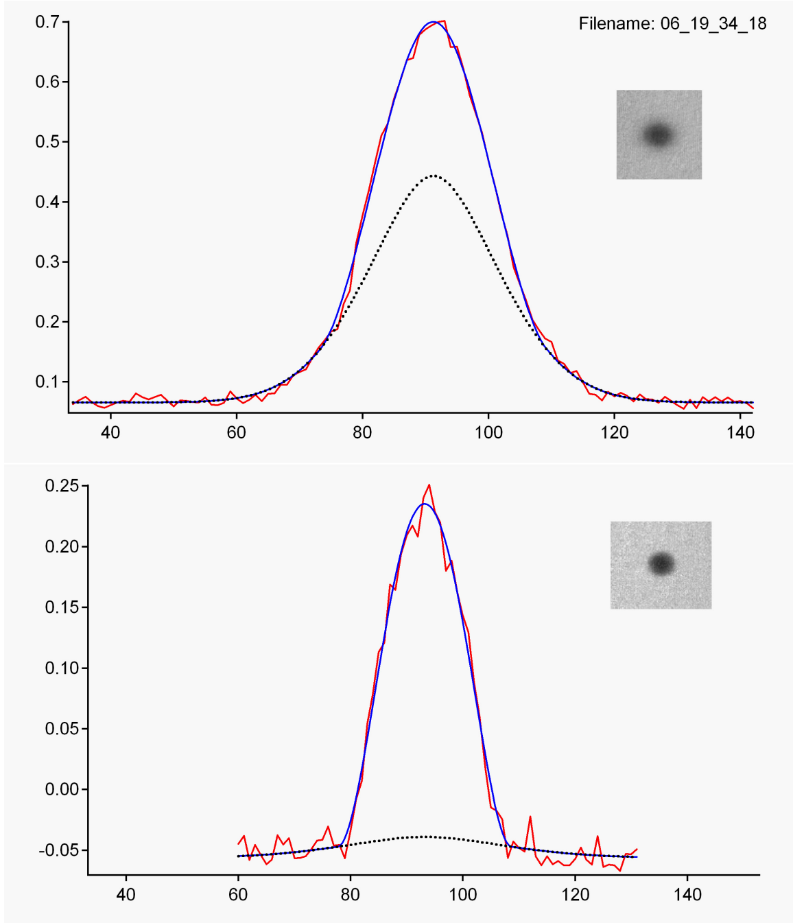
Figure 5-10: The first observation of Bose-Einstein condensate of ^6\text{Li}_2 molecules. This sample was created by evaporating only in the TOT, without transfer into the COT (see text). The temperature of the final condensate obtained can be varied by evaporating to different final optical power. Shown in red jagged lines are density plots of two condensates at different temperatures after ballistic expansion. Solid blue lines are bimodal fits to the data, comprising of a gaussian thermal component (separately plotted in a dashed line) and a Thomas-Fermi fit to the BEC. Top plot shows a condensate emerging from the thermal cloud while bottom plot shows a nearly pure condensate with estimated pair number of 500,000. Insets show absorption images taken along the axial direction.
