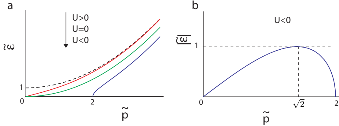
Figure 3-1: (Color in electronic version) Panel (a) shows the dispersion relation (Eq. 3.7) for U > 0 (red), U = 0 (green) and U < 0 (blue) plotted in dimensionless energy and momentum units ( \tilde{\varepsilon} = \frac{\varepsilon}{U} , \tilde{p} = \frac{p}{mc} , c = \sqrt{\frac{U}{m}} ). Dashed line shows the asymptotic form for U > 0 , where the extrapolation down to p = 0 shows an energy offset equal to U . When U < 0 , there exists real eigen-energies only for \tilde{p} > 2 . Panel (b) shows the behavior of |\tilde{\varepsilon}(\tilde{p})| when it becomes imaginary. As discussed, all modes with \tilde{p} < 2 will grow exponentially. For a fixed negative a , there exists a mode |p| which has maximum growth rate.
