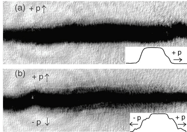
Figure 3-5: Observation of quantum evaporation. Insets show the density profile of a radial slice through the condensate. In (a), a condensate with a > 0 has been seeded with a small population in momentum state p . In time-of-flight, atoms in state p move out of the condensate in a predominantly radial direction. In (b), the interactions in the condensate has been switched to a < 0 after seeding momentum state p . Now \pm p components are seen, with higher population than the initial seed in the +p momentum state.
