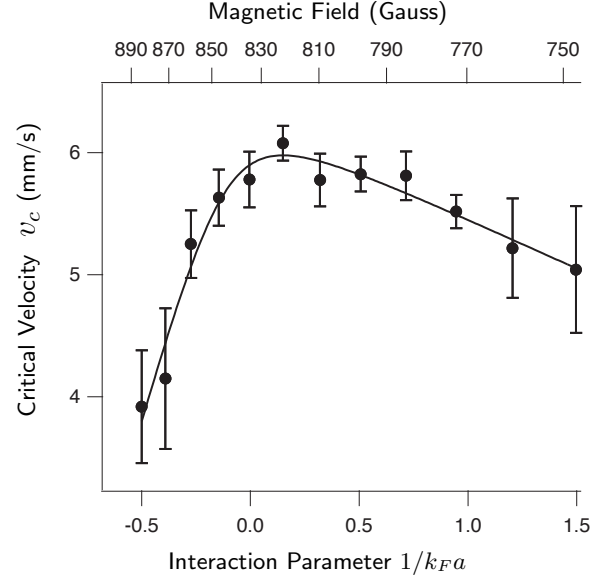
FIG. 2: Critical velocities throughout the BEC-BCS crossover. A pronounced maximum was found at resonance. Data is shown for a V_0 = 0.2 E_F deep lattice, held for t=500 ms. The solid line is a guide to the eye.
