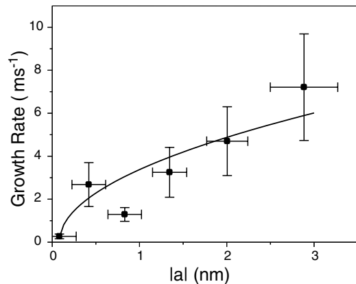
FIG. 4. Growth rate of excitations in a BEC with a < 0 . The rate increases with the magnitude of the negative scattering length |a| . The solid line shows a best fit to the predicted b_1\sqrt{|a|} - b_2 dependence.
