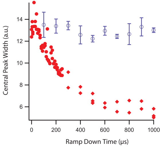
Figure 7-10: Time needed for recoherence. Filled symbols denote the central peak width of the inteferograms. Circles are gaussian widths, while the diamonds are Thomas-Fermi widths obtained from a bimodal fit. Open symbols give the gaussian width of a dephased sample, where phase coherence was deliberately destroyed during the ramp on of the lattice.
