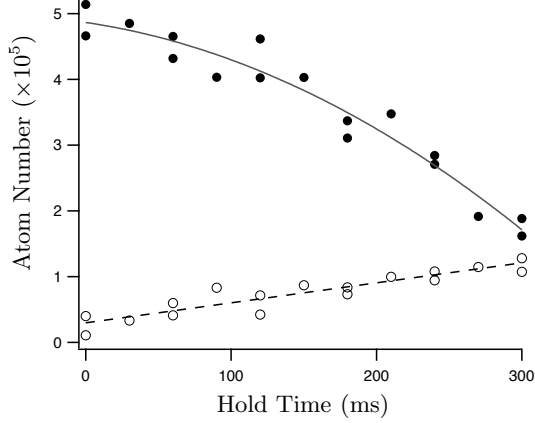
FIG. 5: Number of pairs which remained in the condensate N_c (filled circles) and thermal component N_{th} (open circles) after being held in a V_0 = 0.35 E_F deep optical lattice moving with velocity v_L = 6 mm/s for a variable hold time. The thermal component shows a linear increase (dashed line), whereas N_{cond} showed an accelerated loss, and is fit to a quadratic function (solid line).
