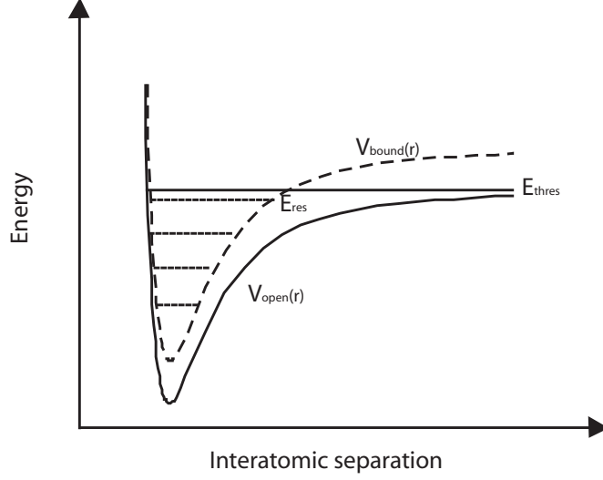
Figure 2-1: An s -wave feshbach resonance occurs when a level crossing between a bound and open scattering channel happens for certain values of the magnetic field. For ultracold collisions, the kinetic energy in the open channel is negligible.
