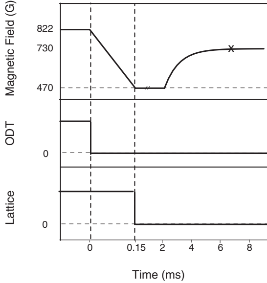
Figure 7-5: The timing sequence that ensures the ballistic expansion for observation of distinct momentum peaks. By quickly ramping to 470 G, strongly interacting {}^6\text{Li}_2 pairs are projected into weakly interacting, deeply bound molecules. The fastest ramp we can achieve is 150\ \mu\text{s} due to technical limitations.
