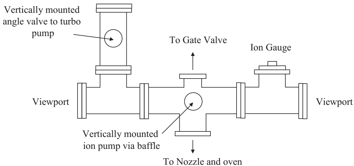
Top View
