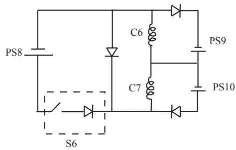
Gradient Coil Wiring Diagram
