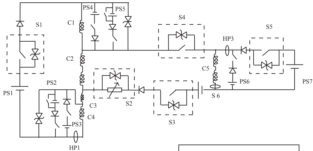
Bias and Curvature Coil Wiring Diagram
