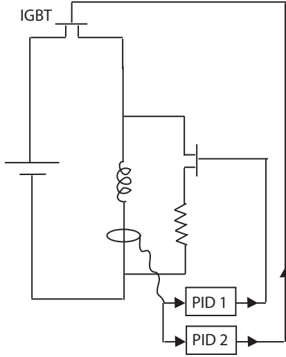
Figure 2-5: Magnetic field stabilization for ^{23}\text{Na} Feshbach work using shunt and total current control. This scheme gave the best transient response for the field (see Fig. 2-6)
