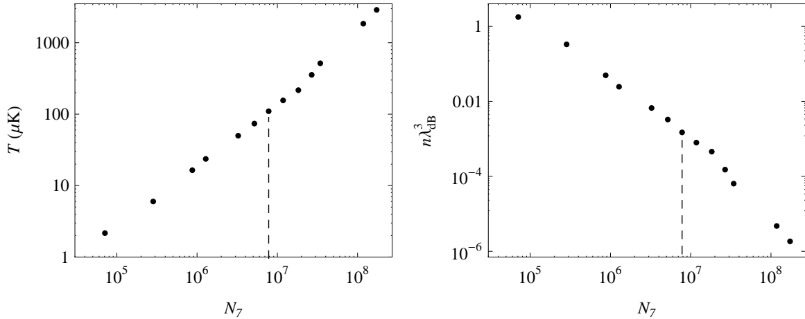
Figure 2.5: Trajectory of ^7\text{Li} forced evaporation: temperature T as a function of atom number N_7 , or peak phase space density n\lambda_{dB}^3(T) as a function of N_7 . The dashed line indicates the evaporation point reached with a maximum ^6\text{Li} atom number N_6 = 5 \times 10^6 (see section 2.3.2).
