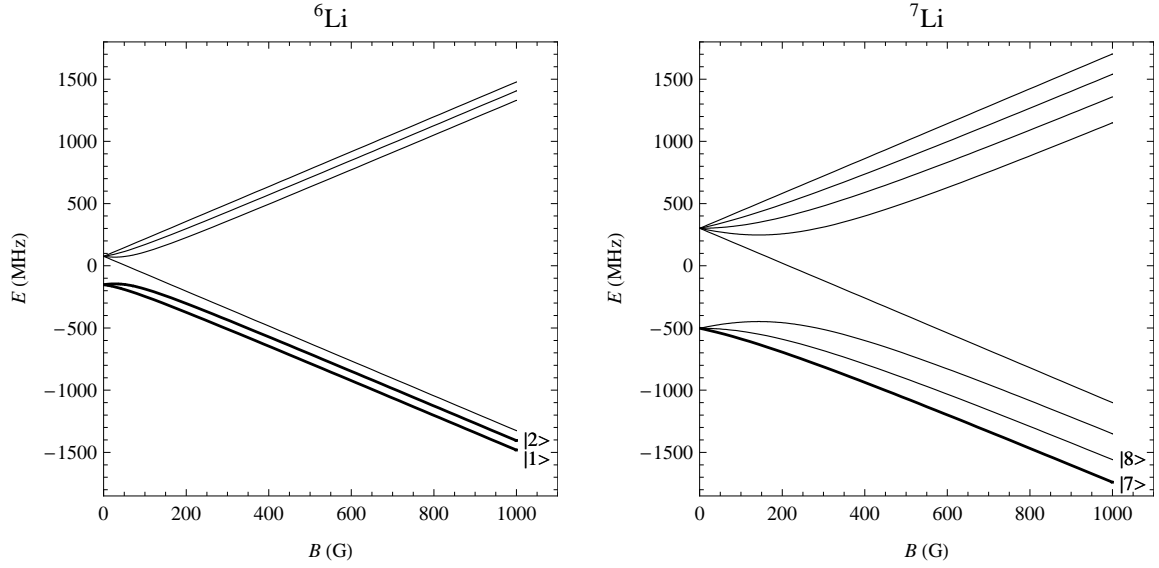
Figure 4.1: Energy levels of the electronic ground state of ^6\text{Li} (left) and ^7\text{Li} (right). The gas is prepared in a mixture of the two lowest states of ^6\text{Li} , labeled |1\rangle and |2\rangle , and of the ground state of ^7\text{Li} , labeled |7\rangle .
