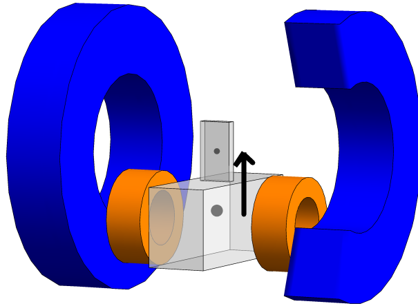
Figure 2.3: Scheme of the magnetic transport. The orange and blue pairs of coils are in anti-Helmoltz configuration.
