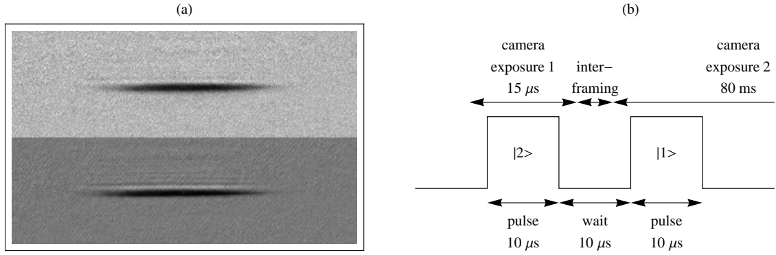
Figure 2.18: (a) Absorption image of a degenerate spin-balanced Fermi gas, using a 100 \mu s pulse (upper panel) and a 10 \mu s pulse (lower panel). The probe intensity is increased by a factor \simeq 10 for the short pulse. The radial sizes are \sigma = 2.3 pixels and \sigma = 1.7 pixels, respectively. (b) Scheme of the imaging sequence for spin-imbalanced gases.
