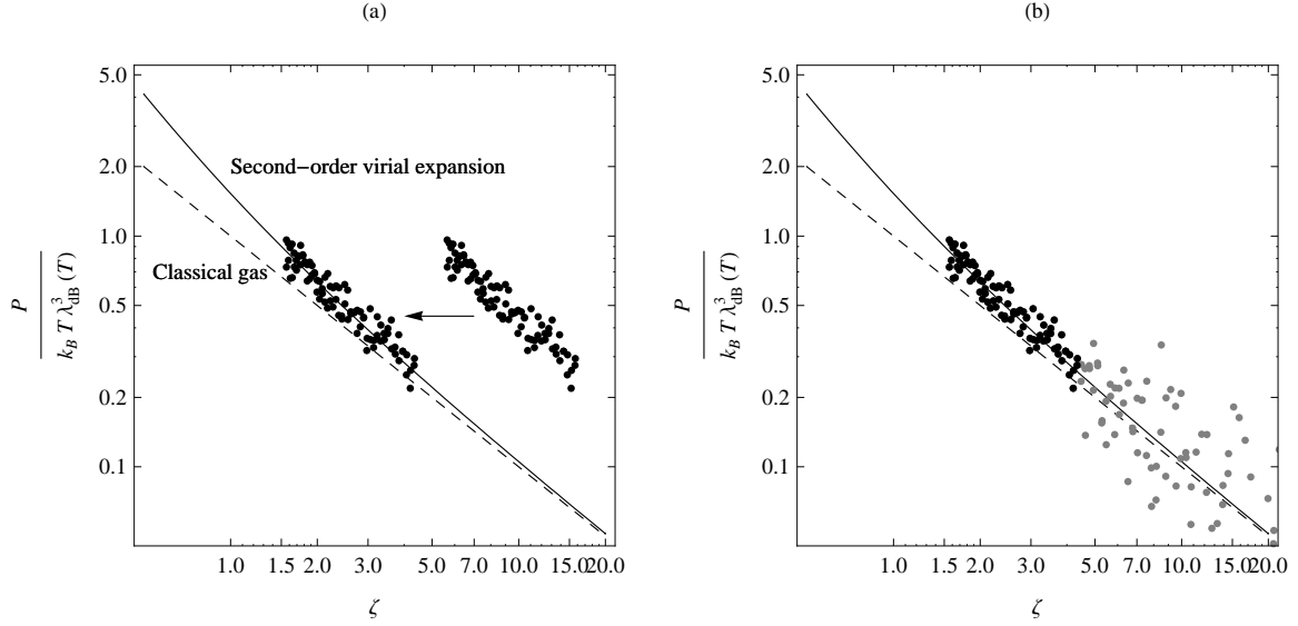
Figure 4.3: (a) The procedure used for the determination of \zeta^0 at high temperature is well illustrated by plotting P(\mu_z, T)/2k_B T \lambda_{dB}^{-3}(T) as a function of \zeta in log scale. Indeed, as \log \zeta = \log \zeta^0 + \log \frac{m\omega_z^2 z^2}{2k_B T} , the degree of freedom \zeta^0 corresponds in that representation to a translation of the data in abscissa. We choose the value of \zeta^0 so that the data corresponding to \zeta_z > 2.5 matches the second-order virial expansion (solid line). The dashed line is the equation of state of a classical ideal gas. (b) Equation of state given by all the pixel columns along the z axis from a high-temperature cloud. For \zeta_z \gtrsim 4 (in gray), the signal-to-noise decreases because of the small optical density in the cloud's wings. We exclude these points for the rest of the data analysis.
