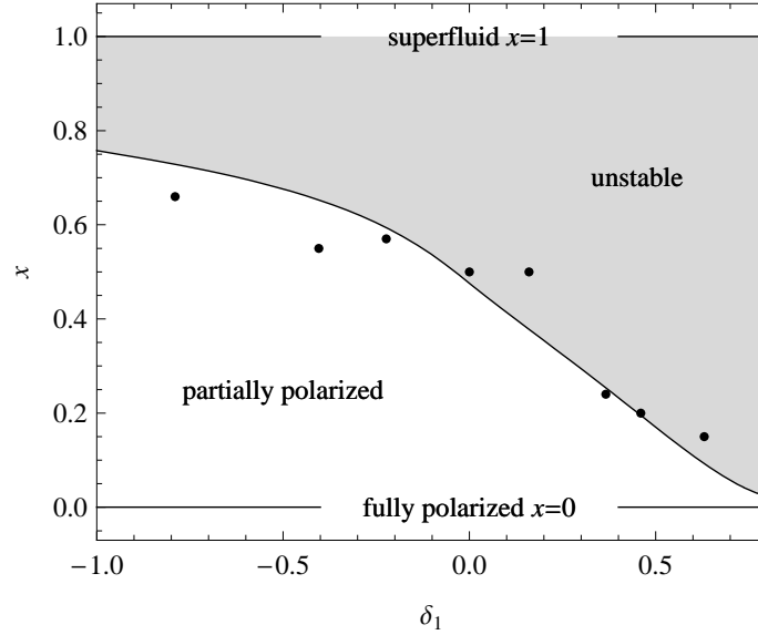
Figure 5.16: Phase diagram of a spin-imbalanced Fermi gas in the (\delta_1, x) plane. The solid line is the maximum minority concentration allowed in the partially polarized phase. The region x_c < x < 1 in gray is thermodynamically unstable.
