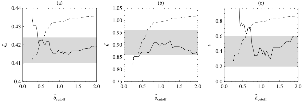
Figure 5.24: Fit results \xi_s (a), \zeta (b) and v (c), as a function of \tilde{\delta}_{\text{cutoff}} . The gray regions indicate our estimation of the actual values of these parameters. The dashed lines are proportional to the number of points used for the fit. When \tilde{\delta}_{\text{cutoff}} is smaller than 0.5, the number of data points becomes small and the fit results strongly depend on the noise of our data.
