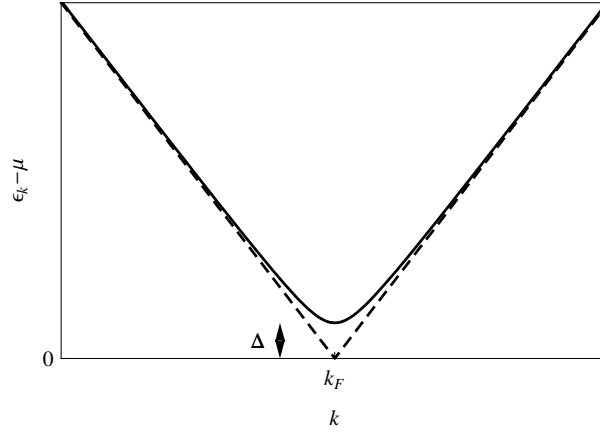
Figure 4.17: Quasi-particle dispersion for a Fermi liquid (dashed line) and with a pseudogap \Delta (solid line)
