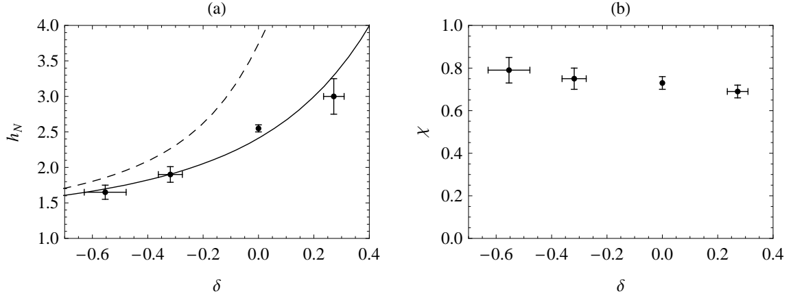
Figure 5.18: (a) Equation of state of the normal phase h_N(\delta) extrapolated to a spin-symmetric configuration (black dots), compared with a fit of the Monte Carlo data from [178] (solid line), and with the superfluid equation of state h_S(\delta) (dashed line). (b) Compressibility \chi(\delta) , normalized to the one of a non-interacting mixture.
