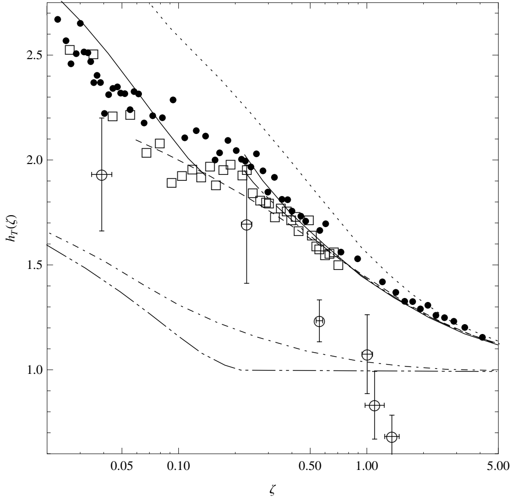
Figure 4.7: Comparison of our data with theory (see text for the legend).
