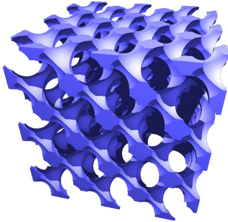
Figure 2. The “inverted diamond” structure was one of the first prototype structures predicted to exhibit a large and robust 3D PBG. It consists of an overlapping array of air spheres arranged in a diamond lattice. This structure can be mimicked by drilling an array of criss-crossing cylindrical holes into a bulk dielectric. The solid backbone consists of a high refractive index material such as silicon leading to a 3D PBG as large as 27% of the center frequency. The minimum refractive index (of the backbone) for the emergence of a PBG is roughly 2.0. Practical difficulties in the synthesis of this structure have motivated simpler but closely related designs such as the “woodpile” structure (see Figure 9 ).
