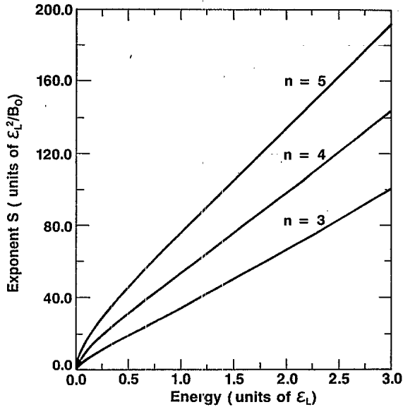
FIG. 4. Same as Fig. 1, except that the autocorrelation functions have the form of B(x) = B_0(1+x^2/L^2)^{-n} . Curves shown are for n=3, 4 , and 5 .
