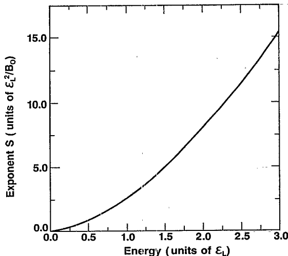
FIG. 5. The calculated S (exponent of the density of states) vs energy for the autocorrelation function of the form B(x) = B_0(1+x^2/L^2)^{-1/2} . The energy unit is \varepsilon_L \equiv \hbar^2/2m^*L^2 .
