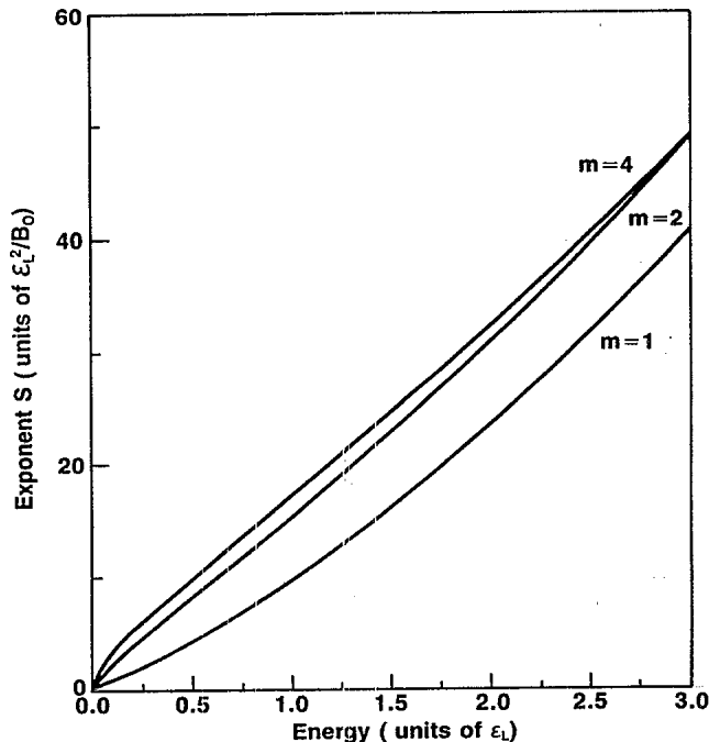
FIG. 1. The calculated S (exponent of the density of states) vs energy for the autocorrelation functions of the form B(x) = B_0 \exp[-(|x|/L)^m] . The energy unit is \epsilon_L \equiv \hbar^2/2m^*L^2 and S is in units of \epsilon_L^2/B_0 . Curves shown are for m=1, 2 , and 4.
