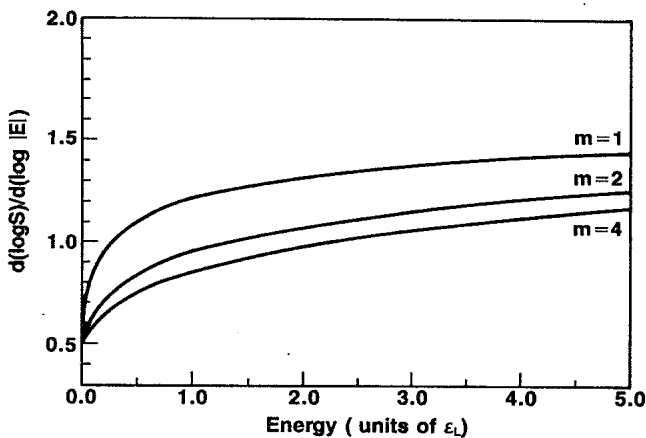
FIG. 2. The logarithmic derivatives n(E) = d(\log S)/d(\log |E|) for the three curves in Fig. 1.
