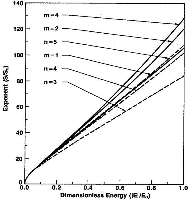
FIG. 6. Results in Figs. 1 and 4 are replotted in the new dimensionless scales E_0 and S_0 to examine the universality. E_0 and S_0 are defined as \hbar^2/2m^*L_0^2 and (1/\gamma_0)E_0^{2-d/2} , respectively, where L_0 is the range of the autocorrelation function (see text) and \gamma_0 \equiv \int d^3x B(x) .
