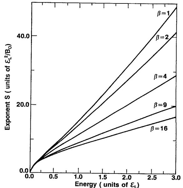
FIG. 3. The calculated S (exponent of the density of states) vs energy for the autocorrelation functions of the form B(x) = [B_0/(1 + \beta^4)](e^{-x^2/\beta L^2} + \beta^4 e^{-\beta x^2/L^2}) . The energy unit is \epsilon_L \equiv \hbar^2/2m^*L^2 . Curves shown are for \beta=1, 2, 4, 9 , and 16.
