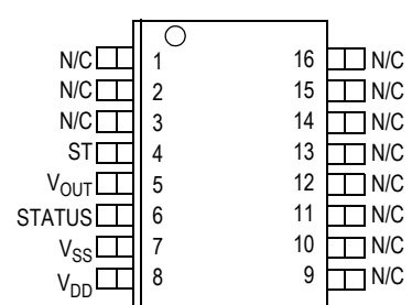
Figure 2. Pin Connections
