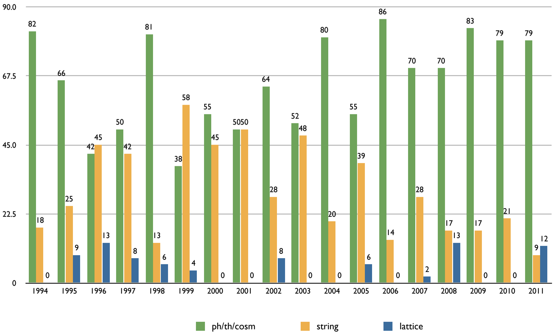
DISTRIBUTION BETWEEN HEP-THEORY SUBFIELDS, AS PERCENTAGE OF TOTAL FACULTY HIRED IN A GIVEN YEAR:
