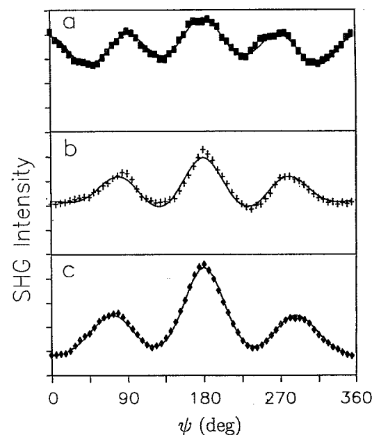
FIG. 1. I_{s,p}^{(2\omega)}(\psi) from the NOS samples with vicinal angles \alpha of (a) 0°; (b) 2°; (c) 5°.
