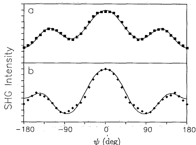
FIG. 3. I_{s,p}^{(2\omega)}(\psi) from the \alpha=5^\circ surface thermally oxidized at (a) 100^\circ\text{C} ; (b) 900^\circ\text{C} .
