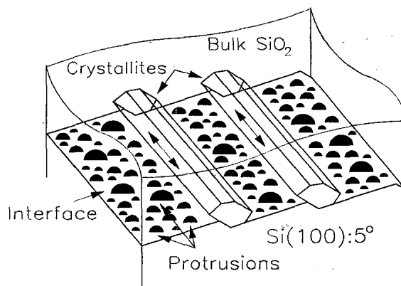
FIG. 5. Schematic representation of our model of the interface after HTO.
