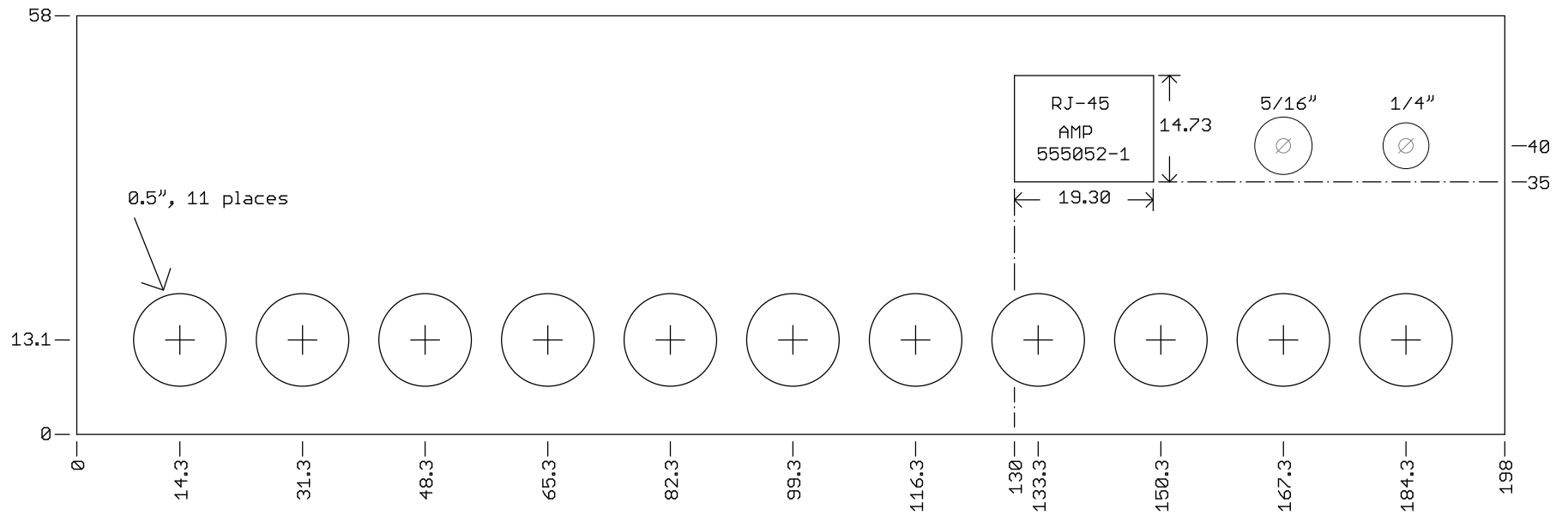
Coincidence Counter, Rev:B, back panel.
