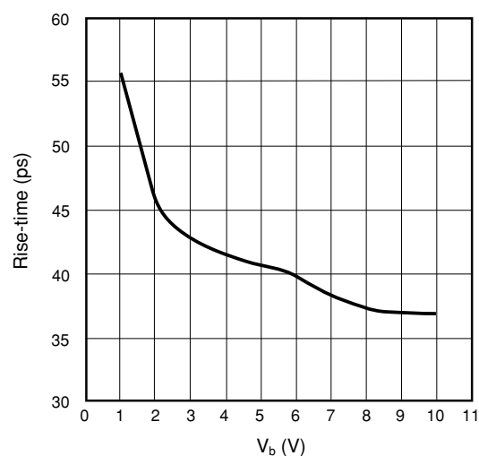
Figure 6: Rise Time vs. Applied Voltage (G7096-03)
