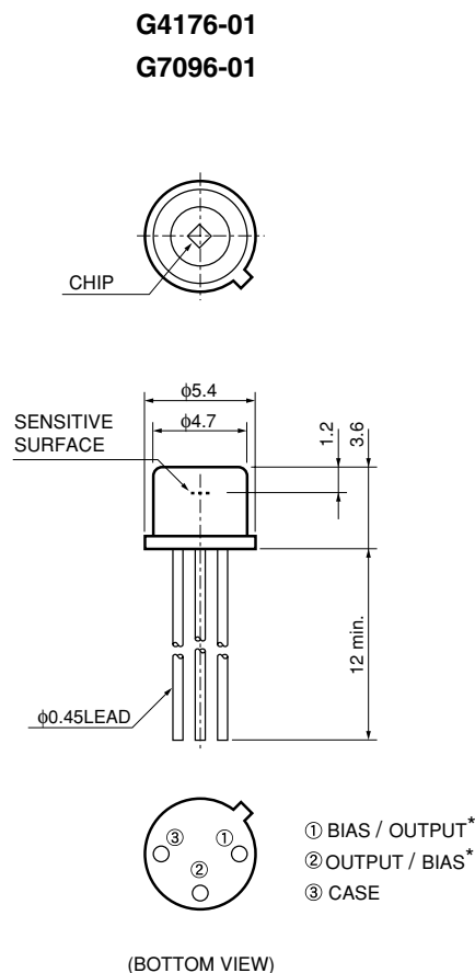
(BOTTOM VIEW)
