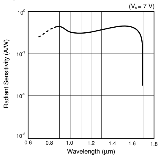
Figure 5: Spectral Response
