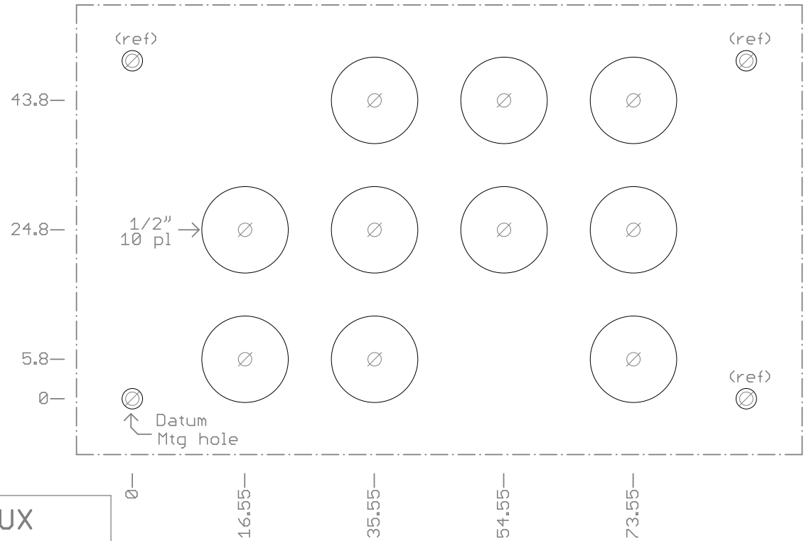
Hammond 1594C drilling (inside view)
