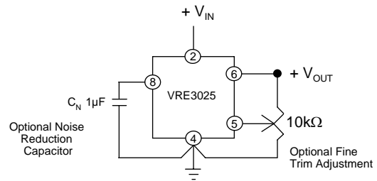
Figure 3 External Connections
