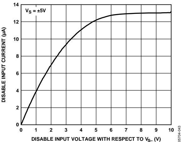
Figure 44. Disable Input Current vs. Disable Input Voltage
