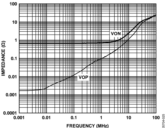
Figure 46. Single-Ended Output Impedance vs. Frequency
