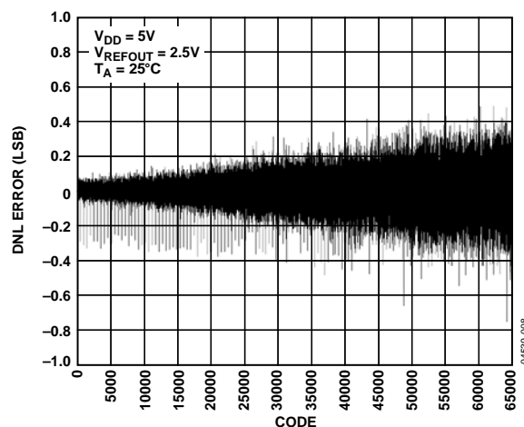
Figure 9. DNL—AD5660-2/AD5660-3
