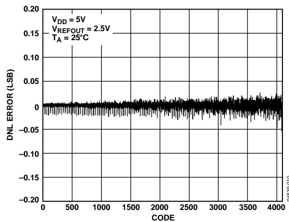
Figure 11. DNL—AD5620-2/AD5620-3
