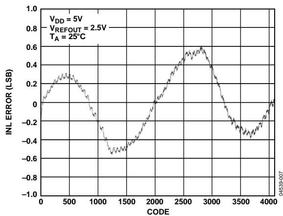
Figure 8. INL—AD5620-2/AD5620-3
