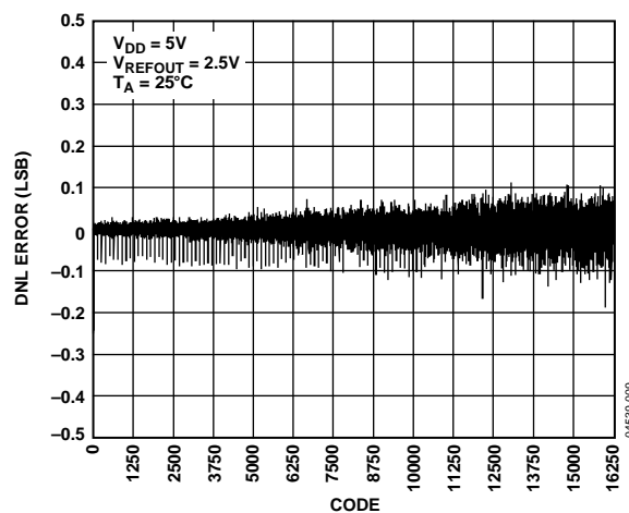
Figure 10. DNL—AD5640-2/AD5640-3
