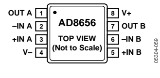
Figure 2. AD8656 8-Lead MSOP (RM-8) 8-Lead SOIC (R-8)
