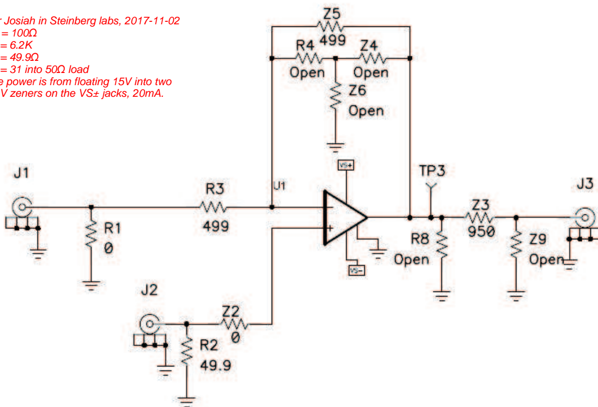
Figure 50. THS4631 EVM Schematic
