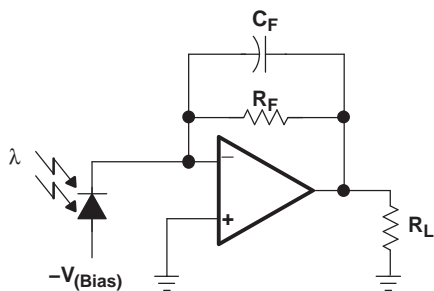
Photodiode Circuit
