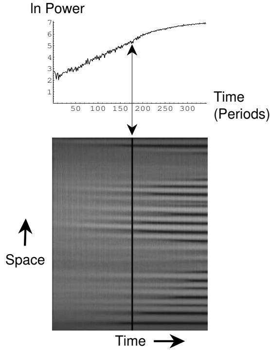
FIG. 3. The exponential growth of the total power in the Fourier spectrum vs. time measured in rotation periods. The loss of exponentiality corresponds to appearance of saturated bands. Here \omega = 3.59 rad/s.
