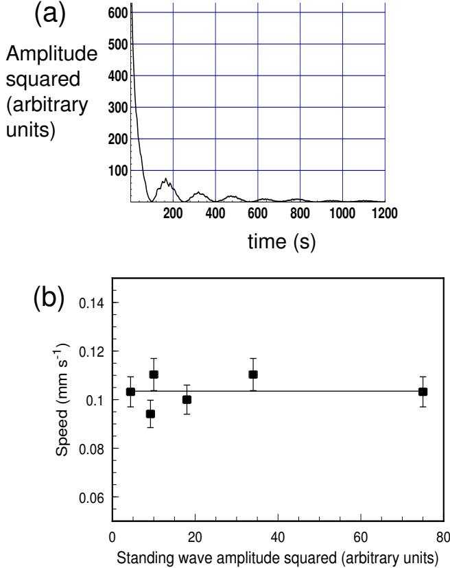
FIG. 10. (a) The amplitude of a standing wave vs. time. (b) The speed of the left- and right-going components of the traveling wave, vs. the peak amplitude squared. Here, \omega = 4.841 rad/s and \phi = 0.67 .
