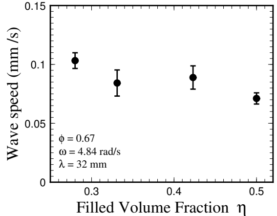
FIG. 11. The traveling wave speed versus the filled volume fraction \eta . The leftmost point corresponds to \eta = 0.28 , which was used for most measurements.
