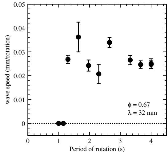
FIG. 12. The traveling wave speed, expressed in mm per rotation period T = 2\pi/\omega vs. the rotation period T . The waves stop traveling for periods of 1.15 s and lower.
