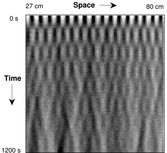
FIG. 7. Standing waves produced by a preseggregated initial condition for \omega = 4.841 rad/s and \phi = 0.67 . Only a portion of the tube is shown.
