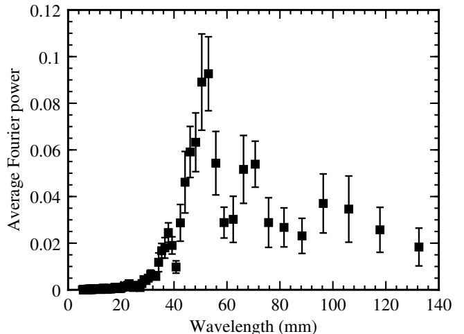
FIG. 5. The Fourier spectrum at the onset of saturation, averaged over the various \omega .
