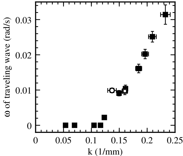
FIG. 8. The dispersion relation for traveling waves at tube rotation frequency \omega = 4.841 rad/s and \phi = 0.67 . The solid symbols indicate presegregated initial conditions. The open symbols are from spontaneous waves using premixed initial conditions, with speeds found from Fourier peaks (open square), and averages of slopes in spacetime images (open circle).
