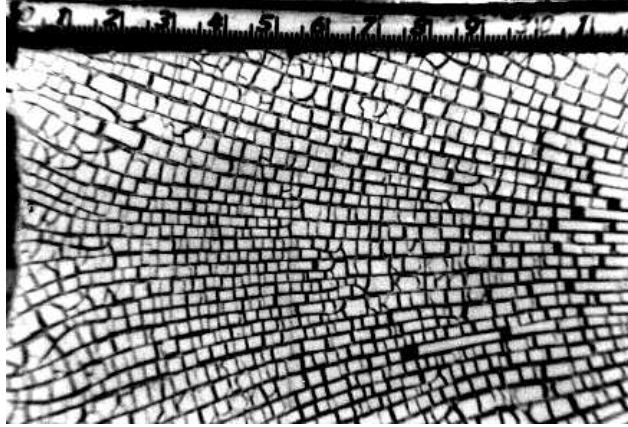
FIG. 2. The crack pattern formed in a directional drying experiment. The substrate was treated with teflon and a sharp drying front moved front left to right across the layer, leaving behind oriented primary cracks. The rungs of the ladder-like pattern are secondary cracks. The front speed was 1.2 mm/hr. Near the middle of the picture, the depth of the layer suddenly increased by about 50%, but no change in the average spacing is evident. This illustrates the weak depth dependence and hysteretic nature of crack spacings on slippery substrates.
