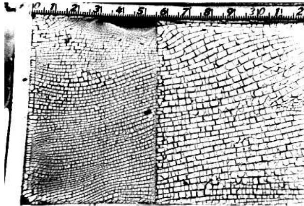
FIG. 7. A directional drying experiment on a rough sandpaper substrate. The sharp drying front moved from left to right across the layer at a speed of 1.5 mm/hr. Near the middle of the picture, the depth of the layer suddenly increases by about 50%, as in Fig. 2. At this point, the crack spacing changes abruptly, approximately doubling.
