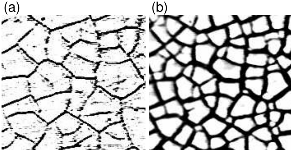
FIG. 3. A portion of the crack pattern forming in a layer 1.31 \pm 0.03 mm thick. Sand has been added to the layer and the substrate was coated with teflon. At least five triplet junctions, formed when three cracks nucleated at a point, are visible in the images. The area shown is 5.7 cm by 5.5 cm. (a) 41 hours into the run. (b) 56 hours into the run.
