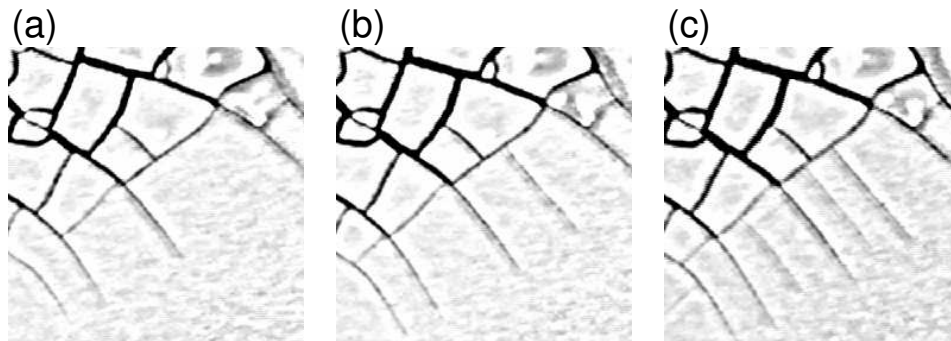
FIG. 7. A directional drying experiment on a rough sandpaper substrate. The sharp drying front moved from left to right across the layer at a speed of 1.5 mm/hr. Near the middle of the picture, the depth of the layer suddenly increases by about 50%, as in Fig. 2. At this point, the crack spacing changes abruptly, approximately doubling.
