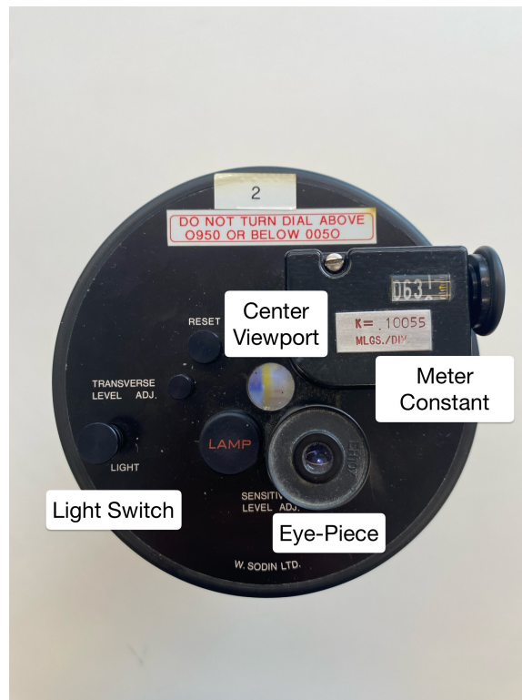
Figure 1: Labeled top view of the gravimeter
