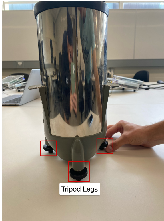
Figure 2: Tripod legs location
