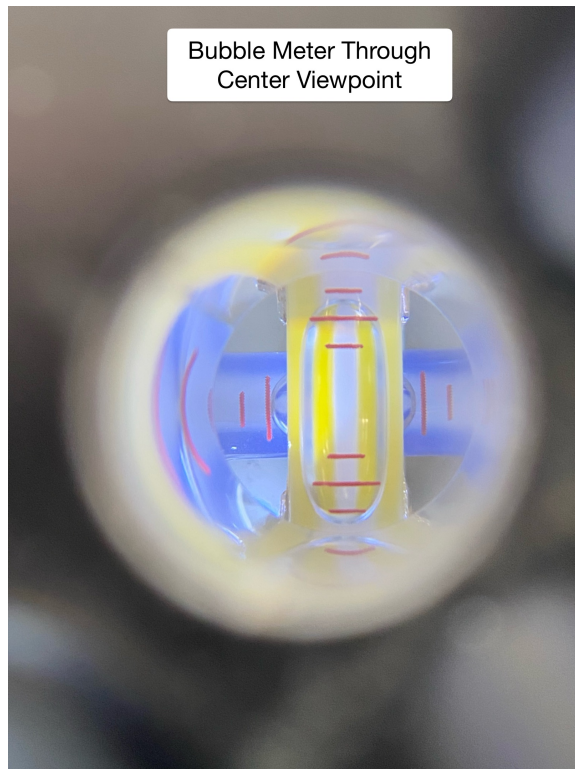
Figure 3: View through the center viewport of the bubble meters aligned correctly.
