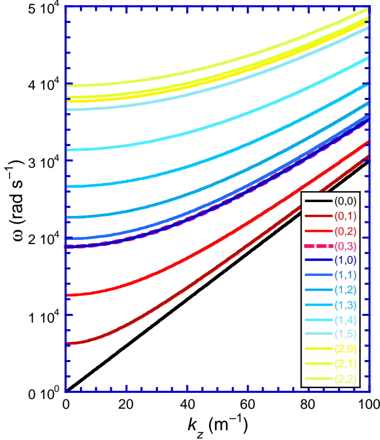
Fig. 1: \omega - k dispersion curve; note modes, labelled in order of increasing cut-off frequency. [needs fix]
