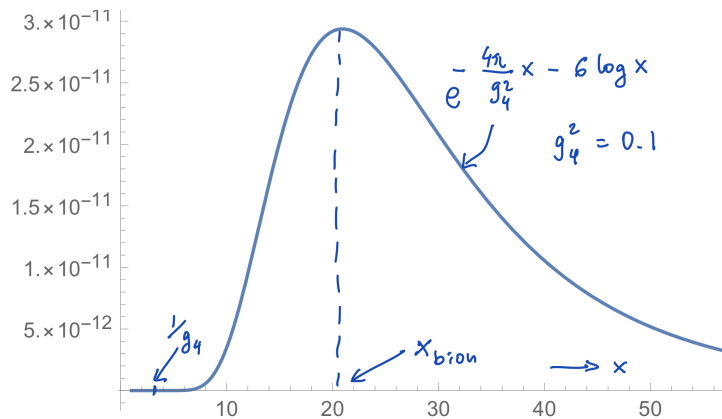
Figure 23: The separation quasizero mode integrand in (125), plotted for g_4^2 = 0.1 and n_f = 2 QCD(adj) in units of L = 1 . The bion size, x_{bion} , is \sim 1/g_4 times larger than the size of the constituent M and KK^* , indicated by 1/g_4 on the figure.
