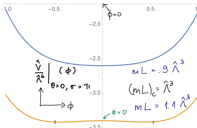
Figure 27: The potential (158) for \sigma = \pi as a function of \phi for two values of mL , above (mL)_c = \hat{\Lambda}^3 (lower curve) with broken Z_2^{(1)} , and below (top curve) with center-symmetric holonomy vev. The top and bottom curve illustrate the 2nd order of the center-symmetry breaking phase transition, corresponding to the unbroken- and broken- Z_2^{(1)} phases, respectively. A study of the \theta -dependence reveals that (mL)_c is a decreasing function of \theta .
