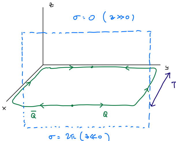
Figure 8: Continuing the Euclidean picture to Minkowski space. Taking x to be the Euclidean time, we intersect the Wilson loop with a fixed-time plane (shown by the dotted line) and plot the resulting field configuration on Figure 9.
