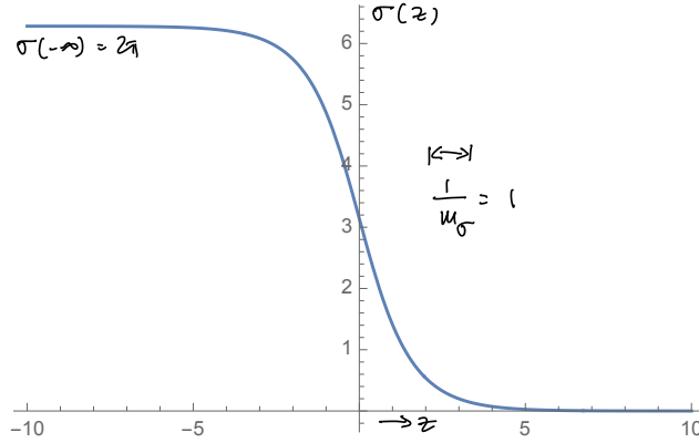
Figure 7: The domain wall solution (51) plotted for m_\sigma = 1 . It is clear that the thickness of the wall is a few times the Compton wavelength of the dual photon, as the naive estimate shows.
