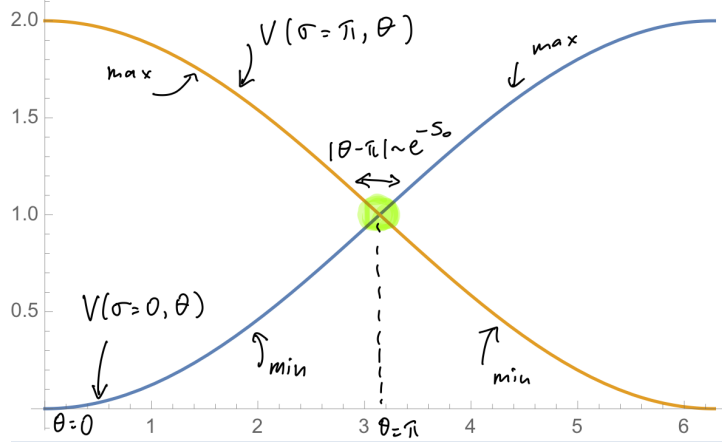
Figure 18: The energies of the two extrema of the leading order semiclassical potential (92), \sigma = 0 and \sigma = \pi , plotted as a function of \theta . At \theta = 0 , the \sigma = 0 extremum is a minimum, while the one at \sigma = \pi is a maximum. Conversely, at \theta = 2\pi , the minimum is at \sigma = \pi , while \sigma = 0 is now a maximum of the potential. The level crossing occurs near \theta = \pi . To study the physics in a finite region |\theta - \pi| = \mathcal{O}(e^{-S_0}) , one has to account of the next order in the semiclassical expansion, due to the fact that the leading-order potential in (92) vanishes at \theta = \pi . As discussed in Section 4.2.1, the next-order contribution implies that there are two ground states at \theta = \pi with broken parity. This reflects the generalized 't Hooft anomaly involving parity and the center symmetry.
