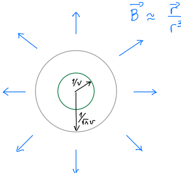
Figure 2: A representation of a monopole-instanton solution in R^3 , showing the scales characterizing the \lambda < 1 spherically-symmetric monopole-instanton: the non-abelian core of size v^{-1} , the outside core region of size (\sqrt{\lambda}v)^{-1} with abelian E_\mu field, and the “long-range” region r > (\sqrt{\lambda}v)^{-1} where only an abelian \vec{B} field in the unbroken- U(1) is present. For our applications, only the long-range region will be relevant, as the monopole-instantons are well separated in the dilute-gas approximation. The action of the \lambda \ll 1 solution is approximately the BPS action (9), S_0 = \frac{4\pi v}{g_3^2} , and the magnetic charge (14) is unity.
