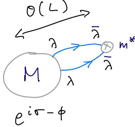
Figure 26: The lifting of monopole-instanton fermion zero modes by a small fermion mass term. The fermion zero modes are localized over a distance of order L , the M size. As m \ll 1/L , the propagators shown by the blue arrows (the same ones responsible for the bion binding of Figure 24) are massless propagators over a distance L , with the divergence cut off by the monopole-instanton core of size L . The calculation is sketched in eqn. (155).
