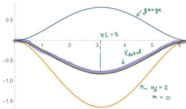
Figure 16: The one-loop effective potential on the Weyl chamber for n_f = 2 massless adjoint fermions, shown by the thick curve (the same L = 1 scale as on Fig. 14 is used). For n_f > 1 , the massless fermions dominate over the gauge contribution in the total potential. The potential on the Weyl chamber is minimized at the center symmetric point \langle \text{tr}\Omega \rangle = 0 . Thus the IR theory is abelian and weakly-coupled at L\Lambda \ll \pi , as discussed in Sections 3.2 and 3.4.1.
