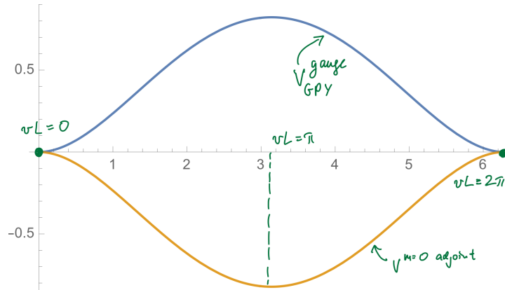
Figure 14: The one-loop effective potential on the Weyl chamber in pure YM theory, computed using supersymmetry (eqn. (81) is plotted with L = 1 ). In the pure-YM theory, the one-loop potential is given by the top curve (81) and the energy is minimized at v = 0 and v = \frac{2\pi}{L} , i.e. at \frac{1}{2} \langle \text{tr } \Omega \rangle = \pm 1 . The Z_2^{(1)} symmetry is thus maximally broken. The physical interpretation of this phase is a deconfined phase of YM theory, see Section 3.4.3.
