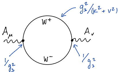
Figure 1: The one-loop heavy W -boson contribution to the photon kinetic term. From (1), all vertices come with a factor \frac{1}{g_3} and the W -boson propagator is \sim \frac{g_3^2}{k^2 + v^2} . Thus, the loop integral scales as \int \frac{d^3k}{(k^2 + v^2)^2} \sim \frac{1}{v} , producing the second term in L_{eff} of (3), with a calculable coefficient C . (For this estimate, the momenta at the interaction vertices can be taken to act on the external A_\mu^3 to produce the field strength in (3)).
