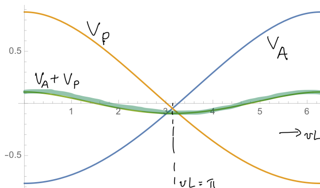
Figure 29: The one-loop holonomy potential (163), the thick line, in an SU(2) gauge theory with a periodic and an antiperiodic massless fundamental flavours. The same scale L = 1 is used, to facilitate comparison with Figures 16 and 17. The P and A contributions, favouring the broken Z_2^{(1)} , are also shown separately.
