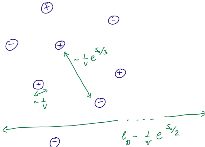
Figure 4: The hierarchy, controlled by the exponentially large e^{S_0} , between the various length scales characterizing the the dilute M - M^* monopole-instanton gas. The dual photon Compton wavelength (the Debye screening length) is the largest length scale. A Debye volume contains a large number of M and M^* fluctuations.
