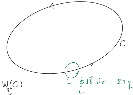
Figure 6: The charge- q Wilson loop W_q[C] requires a 2\pi q monodromy of \sigma around any loop L linked with C . To obtain an analytic expression, we imagine that C is in the xy -plane and take it to be infinitely large, running around the perimeter of the plane.
