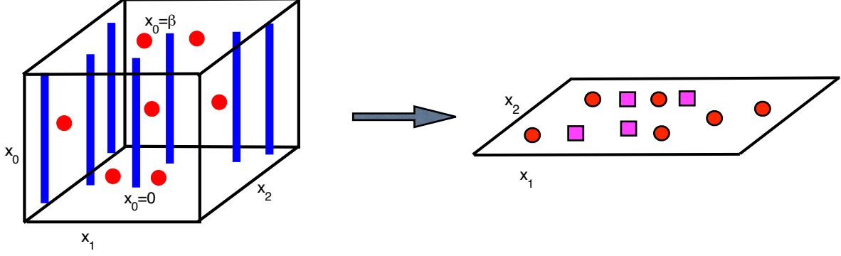
Figure 22: A picture of the R^2 \times S^1_\beta vacuum. The M and KK monopole-instantons, represented by dots, are much smaller than the size of the thermal circle at the temperatures of interest. In addition, static electrically-charged W -bosons, whose worldlines are showed by the blue lines, are excited with nonzero probability. In the temperature range (103), the typical distance between either kind of objects is much larger than the size of the thermal circle (this is not depicted to scale on the drawing and has to be imagined), allowing the gas of to be considered as approximately 2d. The resulting 2d gas of electrically (squares) and magnetically (circles) charged particles is shown on the right. These interact by their respective (magnetic and electric) Coulomb interactions, and also by a mutual Aharonov-Bohm interaction. (Briefly, see the references from footnote 74, the latter is a phase in the Boltzmann partition function that depends on the relative 2d angular positions of the electric and magnetic charges, but not on their distance.) The physics can be studied by various means that we do not have time to discuss, resulting in a deconfinement phase transition at the critical temperature (102).
