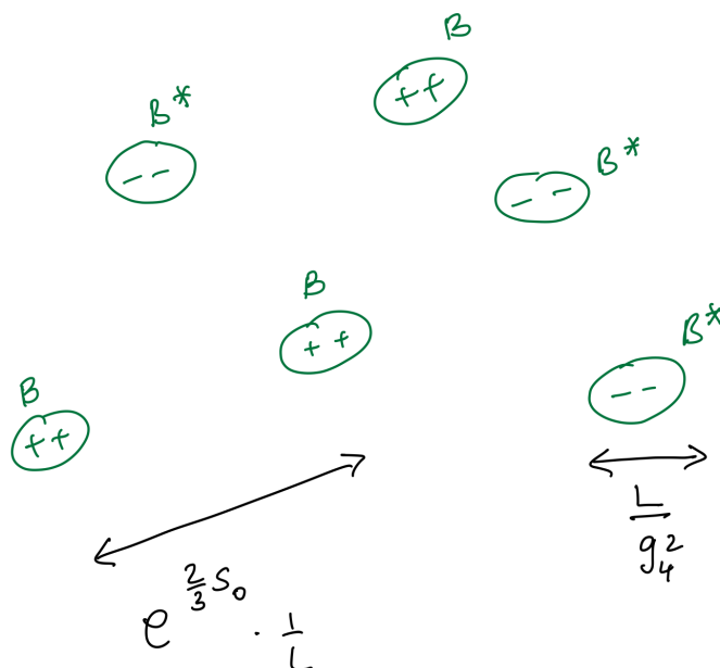
Figure 25: A typical configuration contributing to the vacuum to vacuum amplitude in QCD(adj): a dilute grand-canonical gas of bions B and anti-bions B^* and the hierarchy of characteristic scales involved. Compare with Fig. 4 for the Polyakov model.
