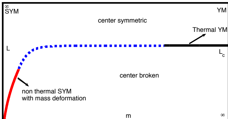
Figure 28: The conjectured phase diagram of softly-broken SYM in the m - L plane. The calculable center-symmetry breaking quantum phase transition, occurring at small- m, L and shown on Figure 27 is in the left-hand corner of the diagram, shown by a thick red line. The center-breaking transition occurs, in the approximation of (158), at the critical value \hat{m} = \hat{\Lambda}^3 . More appropriately, this is written as m = \Lambda^3 L^2 , which is the equation of the thick red curve shown on the plot. If one keeps m fixed, it is clear that the center-broken phase is entered by decreasing L (which, in the thermal theory means going to higher temperature). This weak-coupling quantum phase transition is conjectured to be continuously connected, upon decoupling the gaugino, to the thermal deconfinement transition in pure YM theory, shown by the thick black line on the right.
