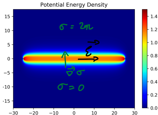
Figure 9: The spatial configuration of static quark/antiquark sources taken at a finite separation, obtained as explained in Figure 8, after taking T to infinity. The potential energy density of the \sigma field is shown. Far from the sources, one can check that the \sigma field profile approaches that of the analytic solution from Figure 7. The gradient of the \sigma field is nonzero only in a flux tube region of width 1/m_\sigma connecting the static sources. In terms of the electric variables, recall the duality relation (21), the \vec{E} -field flux of the sources is collimated in a flux tube (line in R^2 ), the semiclassical confining string of the Polyakov model. (This Figure as well as Figures 19 and 20 are taken from [48, 49] with the sole purpose to qualitatively illustrate the physics, as the Figures are not always for SU(N = 2) . The numerical methods used to obtain them are explained in these references.)
