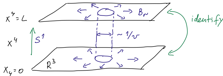
Figure 12: A cartoon of the spacetime structure of the x^4 -independent M monopole-instanton solution on R^3 \times S^1 . This is essentially the solution localized in R^3 shown on Figure 2, now trivially embedded in R^3 \times S^1 , by allowing it to propagate in x^4 without change. The KK monopole-instanton, on the other hand, is twisted in the S^1 direction by the improper gauge transform g_A(x^4) of (59).
